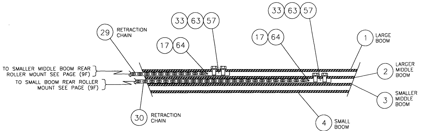
VIEW OF RETRACTION CHAINS MOUNTED TO LARGE & LARGER MIDDLE BOOMS
