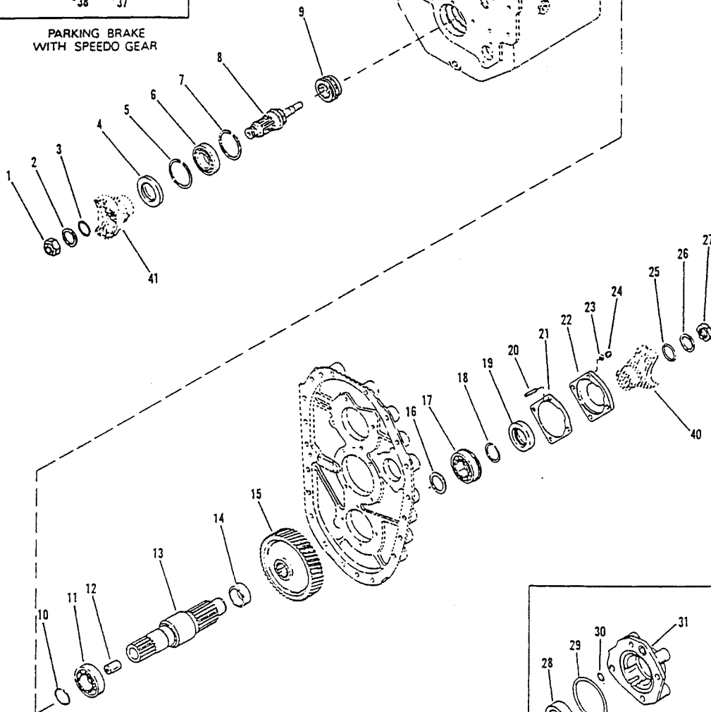
PARKING BRAKE LESS SPEED GEAR
