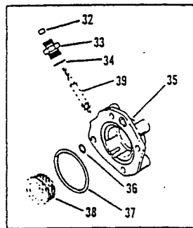
PARKING BRAKE WITH SPEED GEAR
